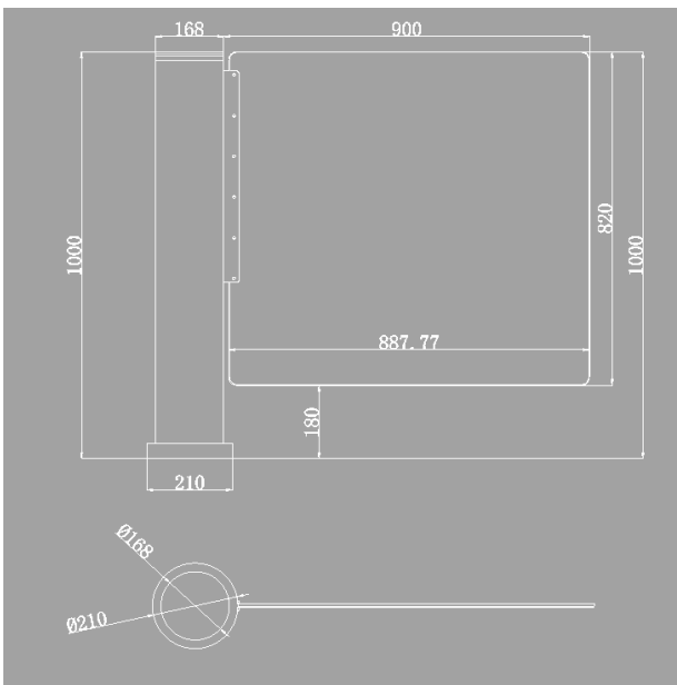
Figure 4 – Product Dimensions
